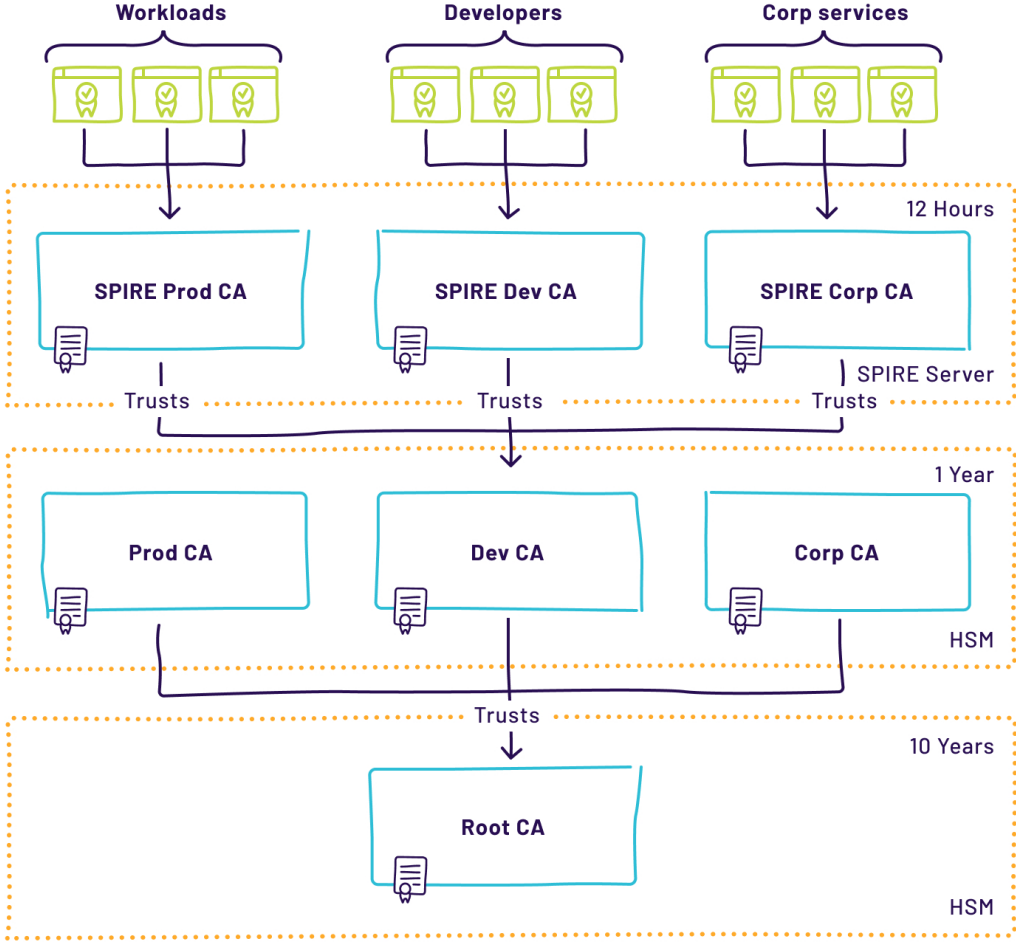
Fig. 6.15: An example SPIRE deployment with three trust domains, each of which uses a different corporate Certificate Authority, each of which uses the same Root Certificate Authority. In each layer, certificates have a shorter TTL.
