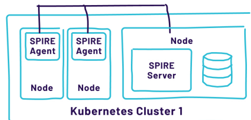
Fig. 6.9: SPIRE Server on the same cluster as workloads.
