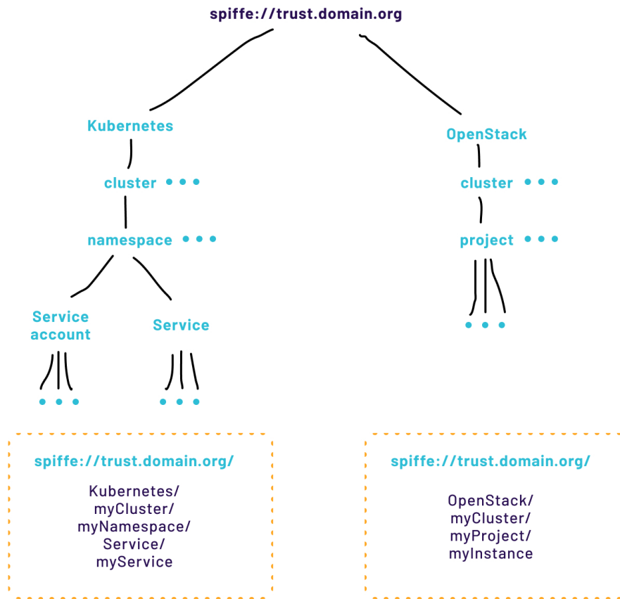
Fig. 8.2: Illustration of another potential SPIFFE ID scheme.
