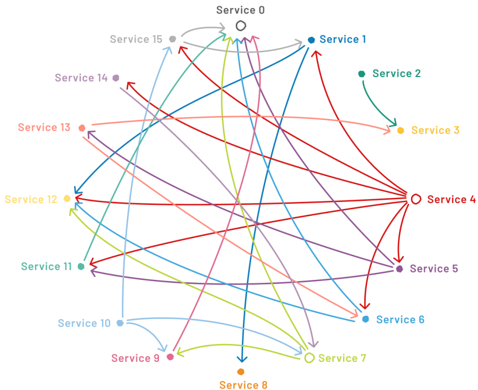
Fig. 5.7: Simplified microservice call graph.
