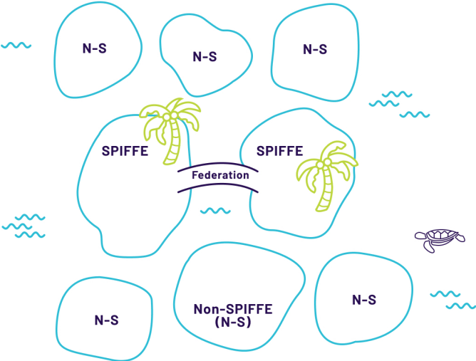
Fig. 5.2: Here we have two independent SPIFFE deployments bridged by Federation, enabling services from each island to trust the other and thereby communicate. There is still no communication between SPIFFE and non-SPIFFE islands.
