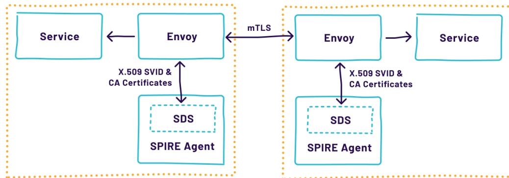
Fig. 7.1: A high-level diagram of two Envoy proxies sitting between two services using the SPIRE Agent SDS implementation to establish mutual TLS.
