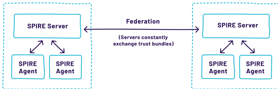
Fig. 4.3: Illustration of a company architecture with two different trust domains connected through the federation. Each SPIRE Server can only sign SVIDs for its own trust domain.
