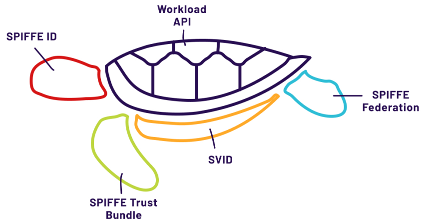
Fig. 4.1: SPIFFE parts.
