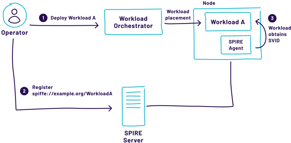
Fig. 6.13: Workload manual registration.
