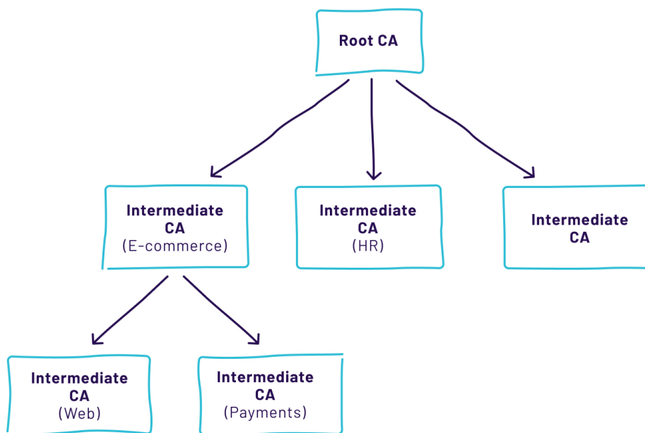
Fig. 3.3: Illustration of intermediate certificate authorities.
