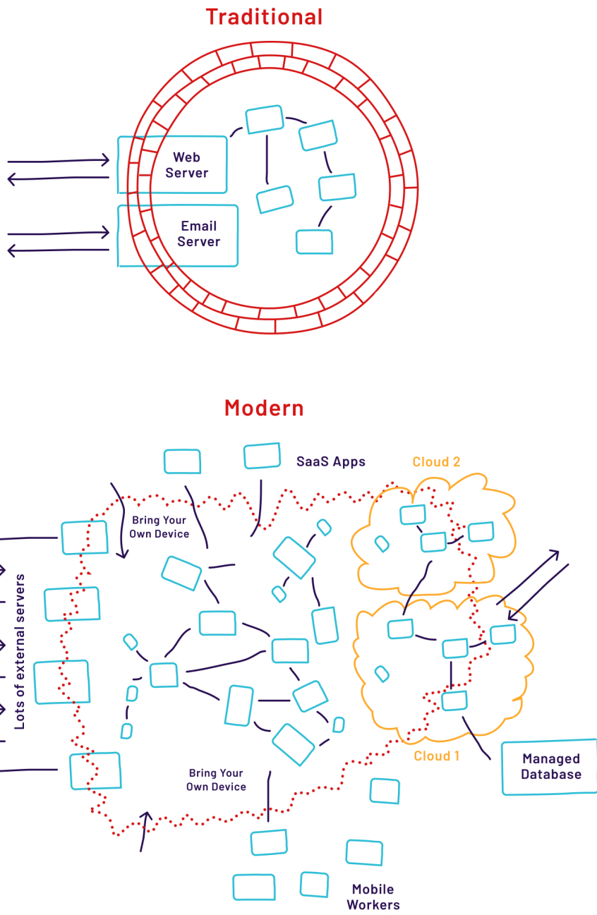
Fig. 1.2: As an organization's networks increase in complexity, adding cloud, SaaS, and mobile workers, building and maintaining perimeter security becomes increasingly unsustainable.
