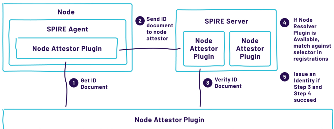
Fig. 6.12: Node Attestor architecture and flow.
