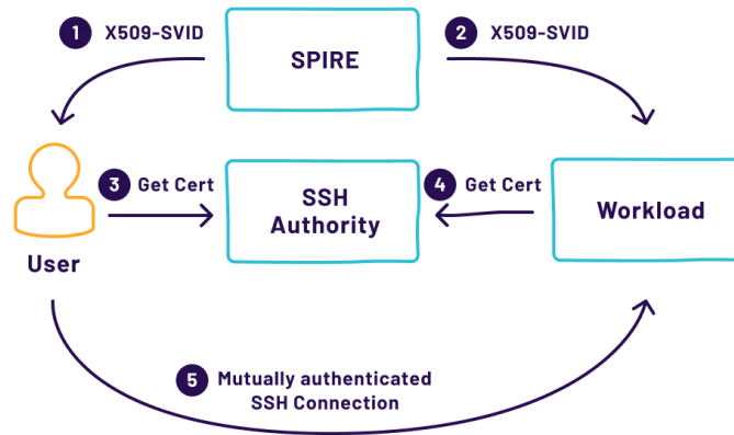
Fig. 7.3: Using SVIDs to bootstrap SSH certificates.
