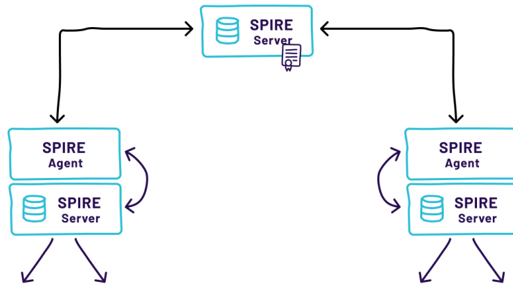
Fig. 6.2: Nested SPIRE topology.
